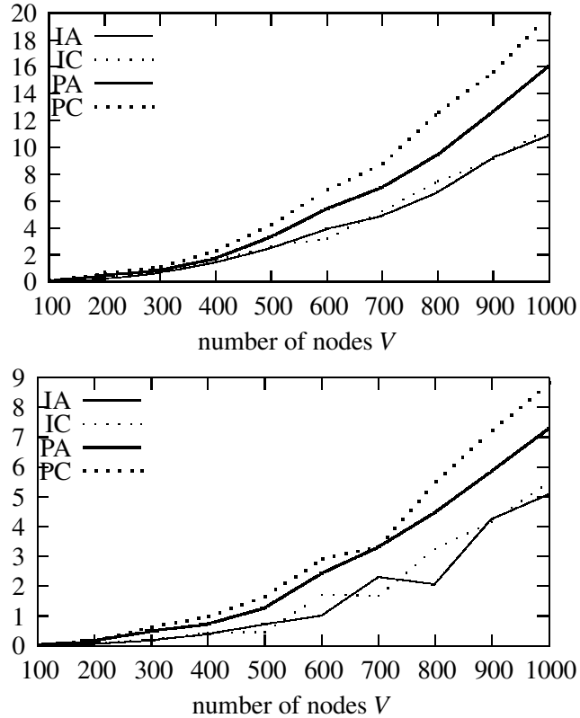
FIGURE 4. Benchmarking creation (top) and deletion (bottom)
