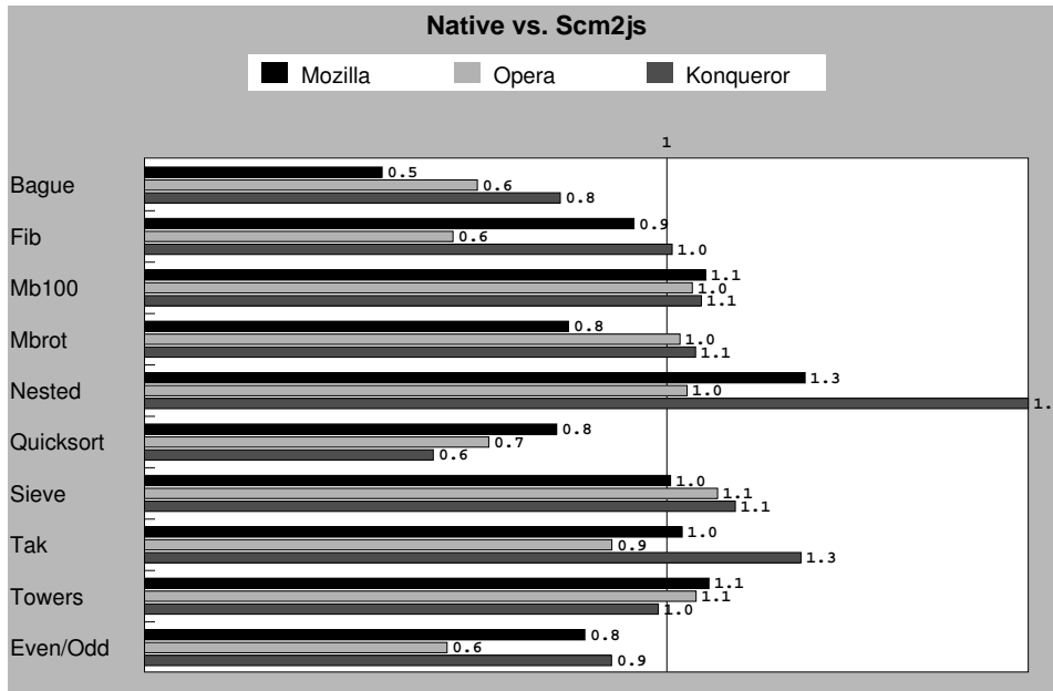
(a) Compiled Scheme relative to handwritten JavaScript files, which are the 1.0 mark. Lower is better.
